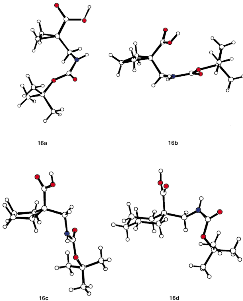
Fig. 1. X-Ray crystal structures of 1-(aminomethyl)cycloalkancarboxylic-acid derivatives 16a–d. Interestingly, the conformation of the urethane C–N bond of compounds 16a , 16b , and 16d is cis (angle O–CO–N–C( \beta ) is sp ). Compound 16c adopts the trans conformation (angle O–CO–N–C( \beta ) is ap ). As expected for the three-membered ring in 16a , the endocyclic angles have values close to 60^\circ , but the CO–C( \alpha )–C( \beta ) angle ( \tau = 117.1^\circ ) is – expectedly so – greater than the standard tetrahedral angle. The angle \tau is 106.5^\circ , 107.0^\circ , and 111.1^\circ in the structures of compounds 16d , 16c , and 16b , respectively. For structure determination of compound 16c we thank Dr. W. B. Schweizer.
